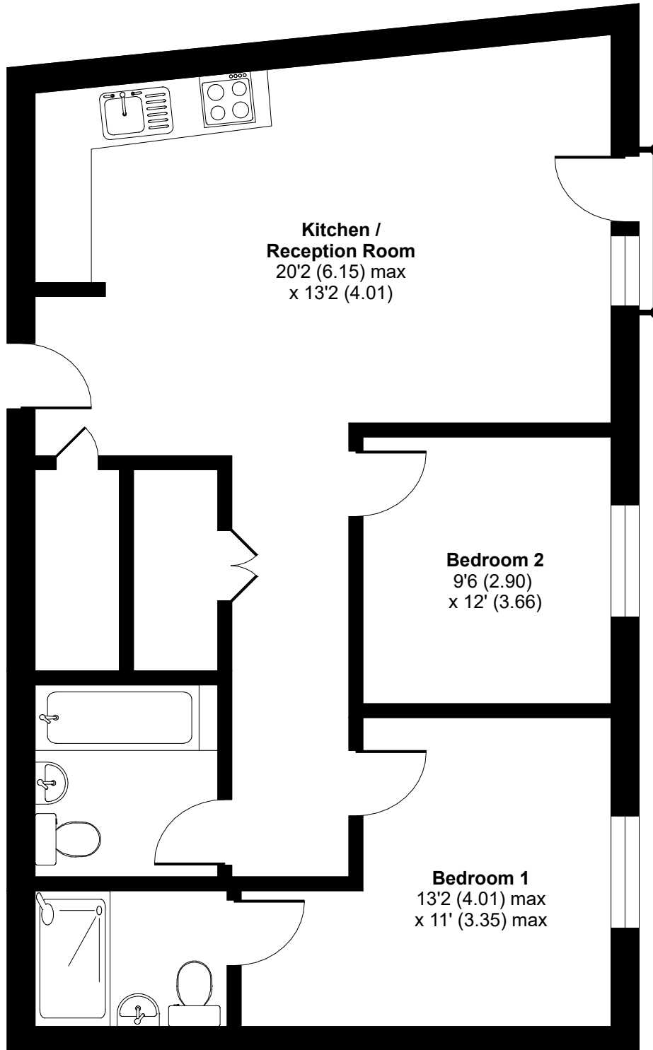
SECOND FLOOR
